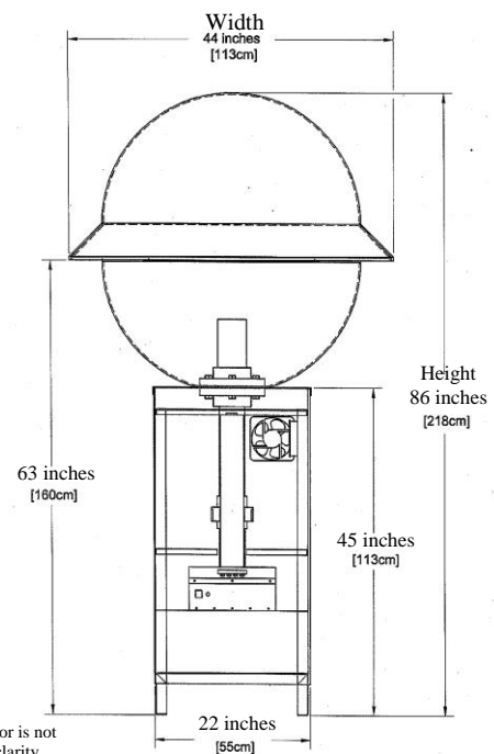
Dimensional Sketch
